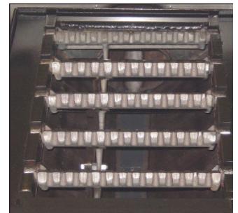
Shaker grates (open).
